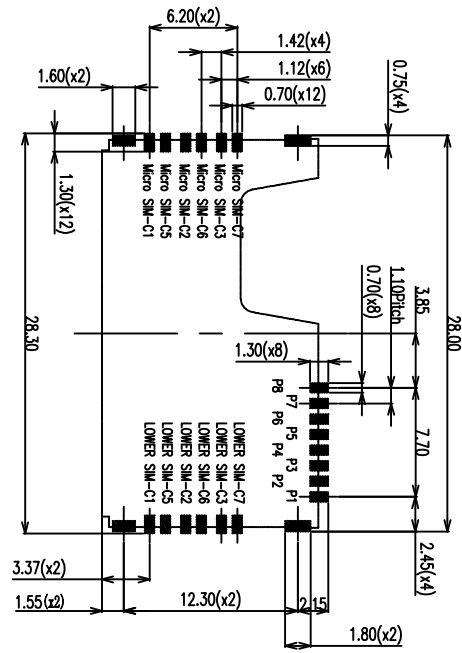
RECOMMENDED PCB LAYOUT TOLERANCES ±0.05(TOP VIEW)
