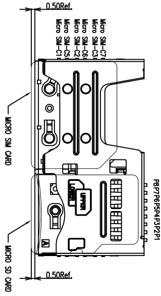
MICRO SIM CARD & MICRO SD CARD PIN NO.(SEE TABLE B)
